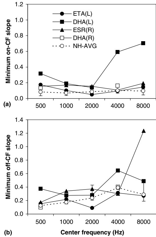
Fig. 7. Minimum growth rates (minimum slopes) of the estimated BM response functions for tones at CF (a) and well below CF (b) (measured from the response functions shown in Figs. 5 and 6). Filled symbols: HI ears; open symbols: NH ears. Open circles illustrate corresponding values for the average response functions for three NH listeners. Error bars are associated to the open circles and illustrate the range of individual values for three NH listeners.
