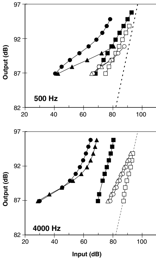
Fig. 6. Inferred BM response functions for the NH [DHA( r ), circles] and HI [DHA( l ), squares] ears of unilaterally HI listener DHA. Also shown are the response functions for the average of three NH listeners (triangles) (adapted from Lopez-Poveda et al., 2003). Filled symbols: responses for tones at CF; open symbols: responses for tones an octave below CF. Top panel: CF = 500 Hz; Bottom panel: CF = 4000 Hz.
