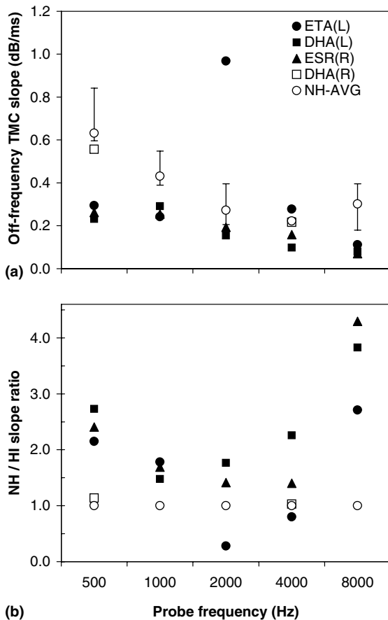
Fig. 4. (a) Slope (dB/ms) of straight lines fitted by least squares to the off-frequency TMCs for the three HI ears (filled symbols) and the NH ear (open squares) tested here. Open circles illustrate the slopes for the average off-frequency TMCs for the three NH listeners in Lopez-Poveda et al. (2003). Error bars are associated to the open symbols and illustrate the range of slope values for the individual TMCs reported in that same study. (b) Ratio of the slopes for the average NH listeners over the slopes for the each of the HI ears (filled symbols) and the NH ear (open squares) tested in the present study. Note that the off-frequency TMCs are almost always steeper for the NH than for the HI ears.
