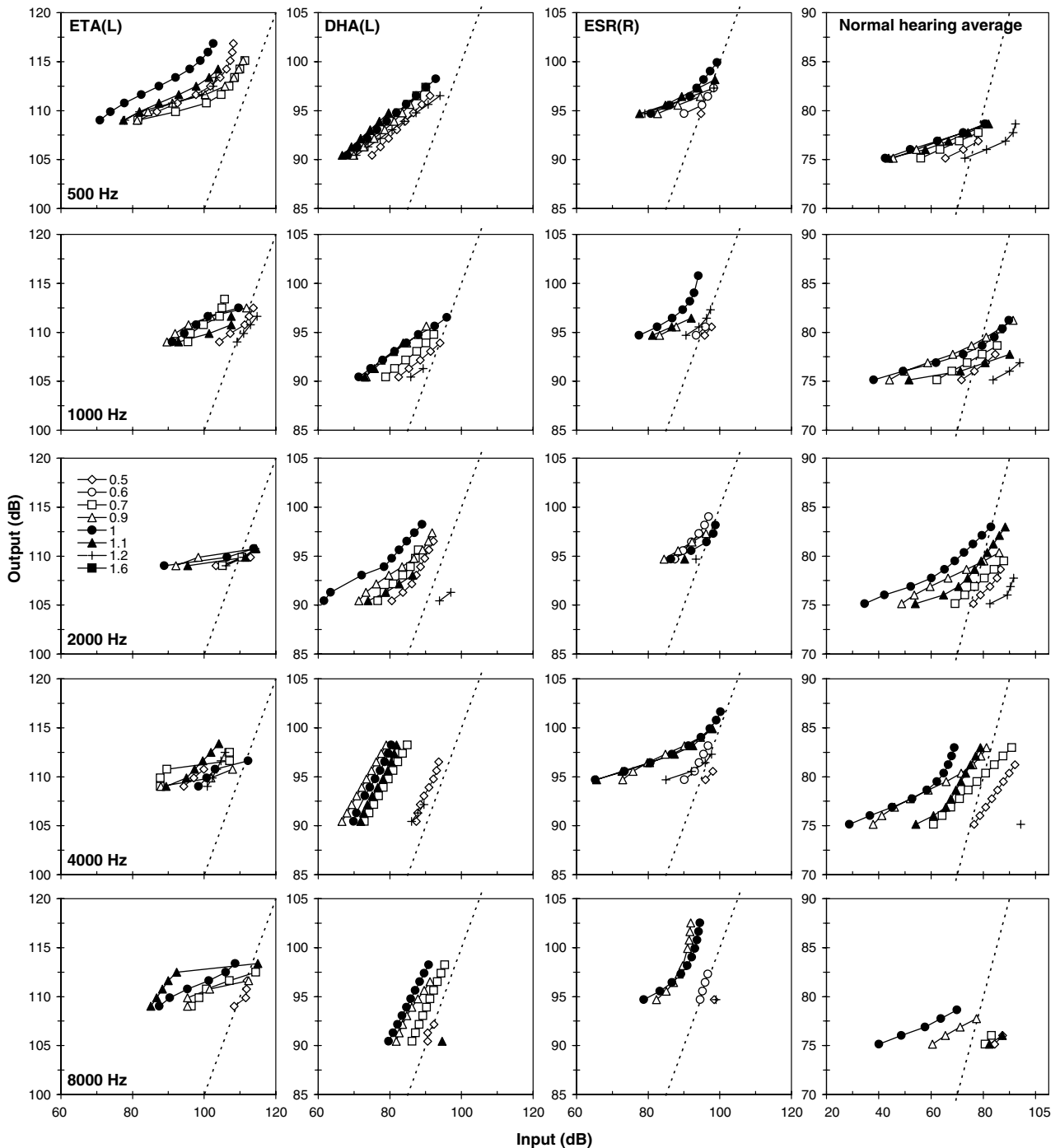
Fig. 5. Inferred BM response functions. Each column illustrates the response functions of a different HI listener or the average of three NH listeners (right-most column). Each row corresponds to a different center frequency from 500 Hz (top row) to 8000 Hz (bottom row). The inset in the mid panel, left column informs of the stimulation frequencies relative to CF. Dotted lines illustrate a perfectly linear response with zero gain.
