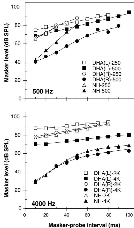
Fig. 3. TMCs for the NH ear, DHA( r ), and the HI ear, DHA( l ), of unilaterally HI listener DHA. Average TMCs for three other individuals with NH are also shown (triangles) for comparison (adapted from Lopez-Poveda et al., 2003). Top panel: TMCs for a probe frequency of 500 Hz and masker frequencies of 250 and 500 Hz. Bottom panel: TMCs for a probe frequency of 4000 Hz and masker frequencies of 2000 and 4000 Hz. The numbers in the legend indicate the masker frequency. Note that the TMCs for DHA( r ) match closely the average NH TMCs for all conditions except for the on-frequency 500-Hz TMC. For this condition, the TMC for DHA( r ) is shallower than normal. The TMCs for HI ear, DHA( l ) (squares), are shallower than the TMCs for the NH ears (circles and triangles), both for on (filled symbols) and off-frequency maskers (open symbols) (Fig. 4). The continuous lines illustrate example fits of Eq. (1) to the TMCs. Note that the fits are generally very good.
